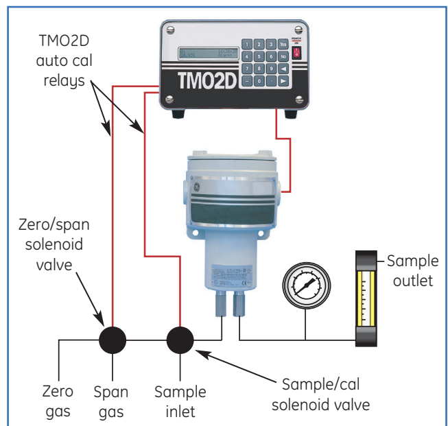
TMO2D with XMO2 and sample system
